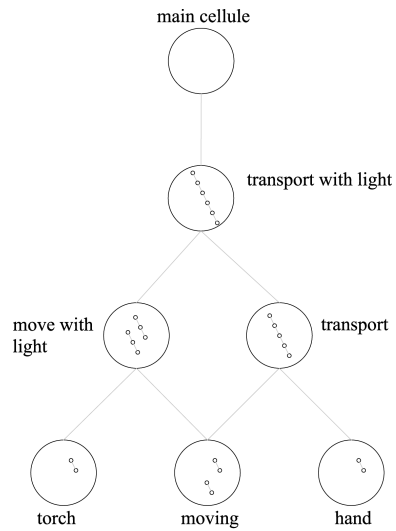
Figure 4.3: Construction of the cell tree. Phase 5
