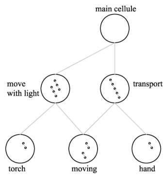
Figure 4.2: Construction of the cell tree. Phases 3 (up) and 4 (down).
